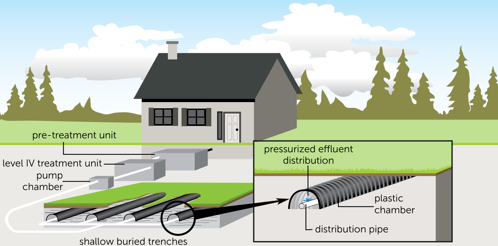
Figure 9. Shallow buried trenches provide distribution back into the native soil for additional treatment.
