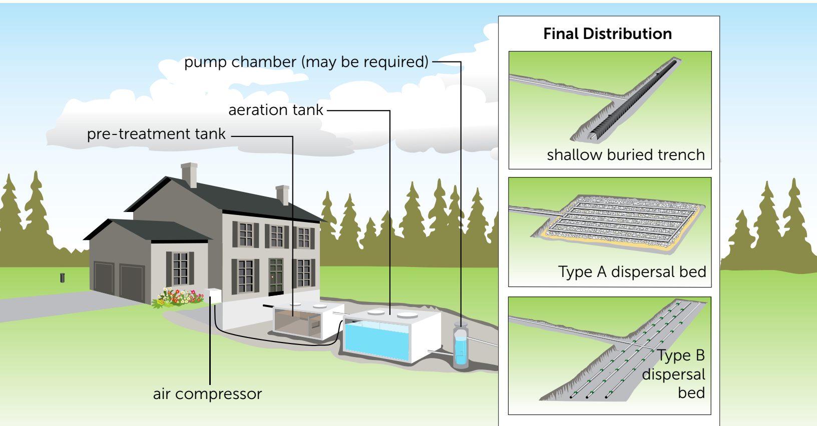
Figure 7. Aerobic treatment units provide Level IV effluent treatment. This allows for a final distribution system that has a smaller footprint.
