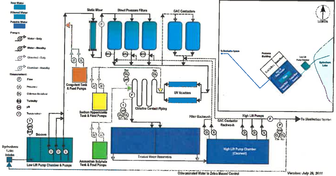
SYDENHAM WATER TREATMENT PLANT PROCESS FLOW
